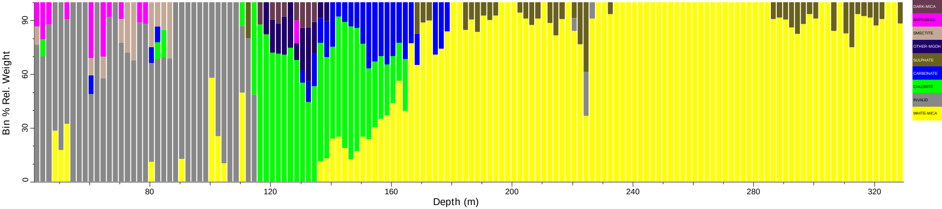
09THD028_tsg_tir: Spatial Summary (Bin=2 MinBin=5% sjCLST 7.08)
