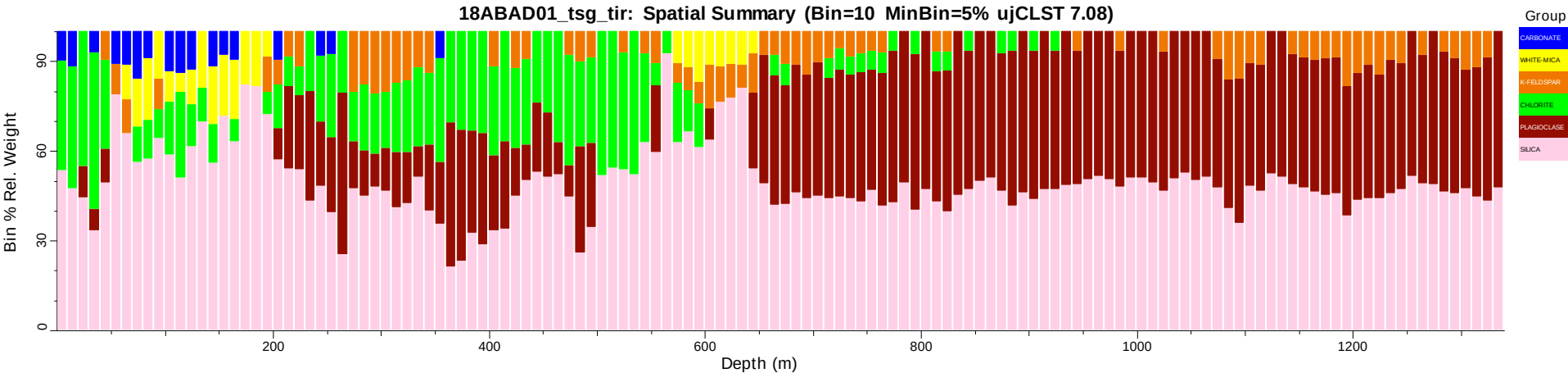
18ABAD01_tsg_tir: Spatial Summary (Bin=10 MinBin=5% ujCLST 7.08)
