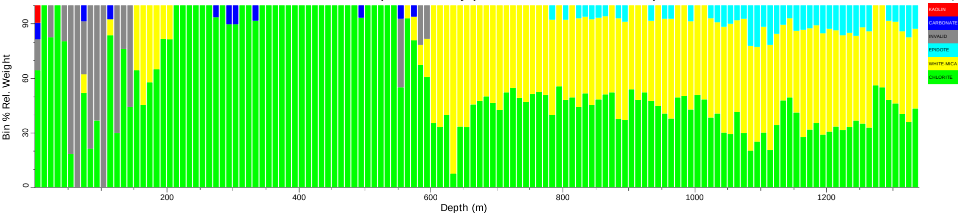
18ABAD01_tsg_tir: Spatial Summary (Bin=10 MinBin=5% ujCLST 7.08)
