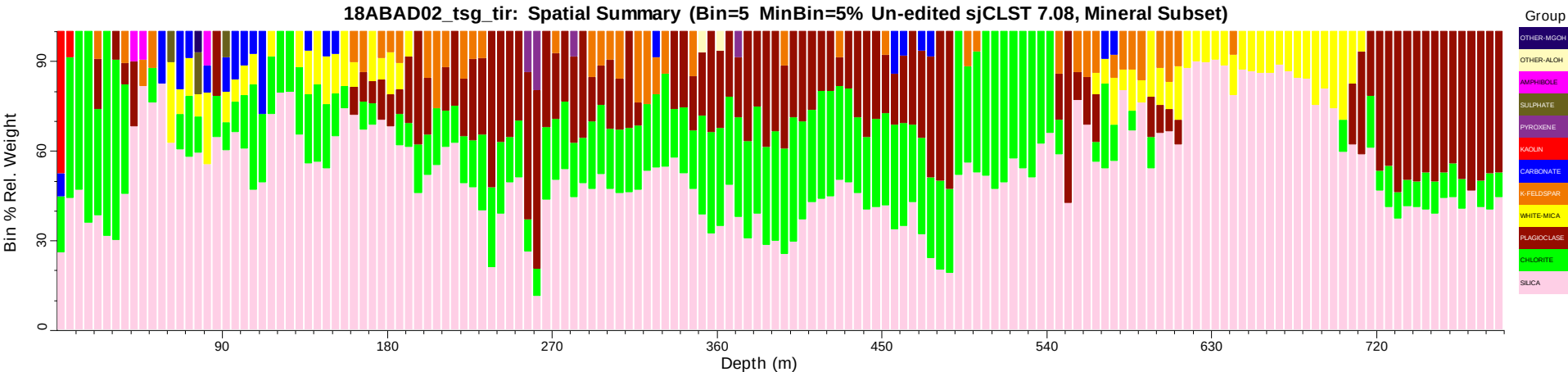
18ABAD02_tsg_tir: Spatial Summary (Bin=5 MinBin=5% Un-edited sjCLST 7.08, Mineral Subset)
