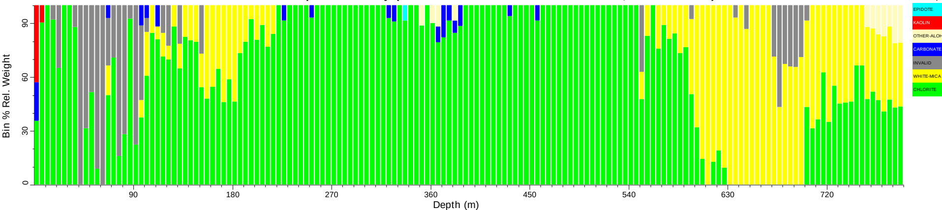
18ABAD02_tsg_tir: Spatial Summary (Bin=5 MinBin=5% Un-edited sjCLST 7.08, Mineral Subset)
