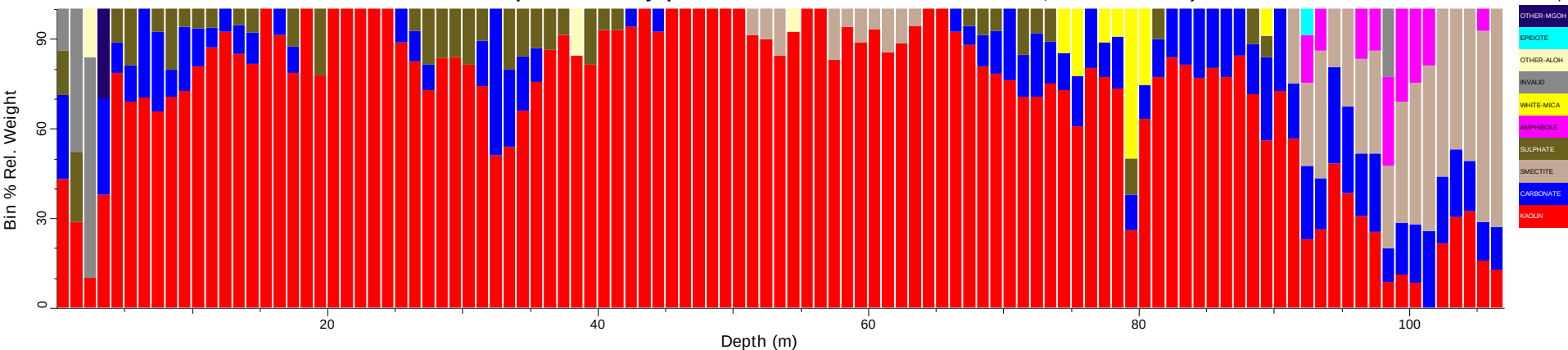
19MODD022_tsg_tir: Spatial Summary (Bin=1 MinBin=5% Un-edited sjCLST 7.08, Mineral Subset)
