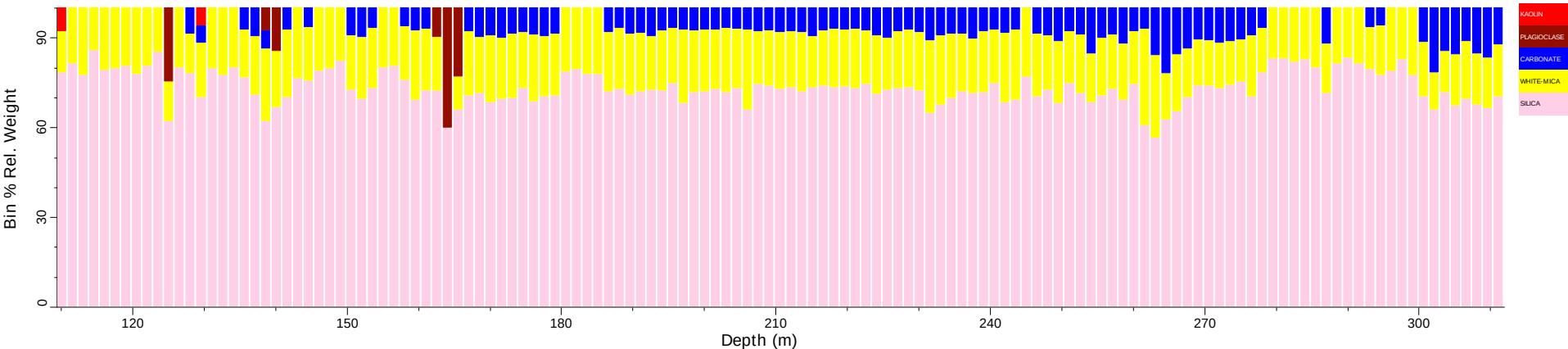
21MBRCD042_tsg_tir: Spatial Summary (Bin=1.5 MinBin=5% Un-edited sjCLST 7.08, Mineral Subset)
