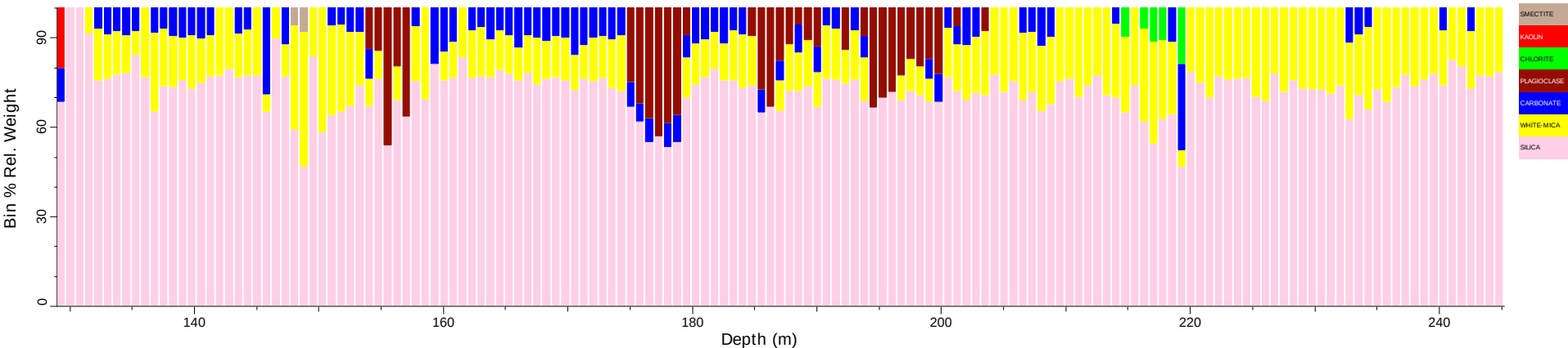
21MBRCD043_tsg_tir: Spatial Summary (Bin=0.75 MinBin=5% Un-edited sjCLST 7.08, Mineral Subset)
