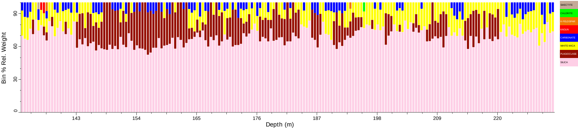
21MBRCD044_tsg_tir: Spatial Summary (Bin=0.5 MinBin=5% Un-edited sjCLST 7.08, Mineral Subset)
