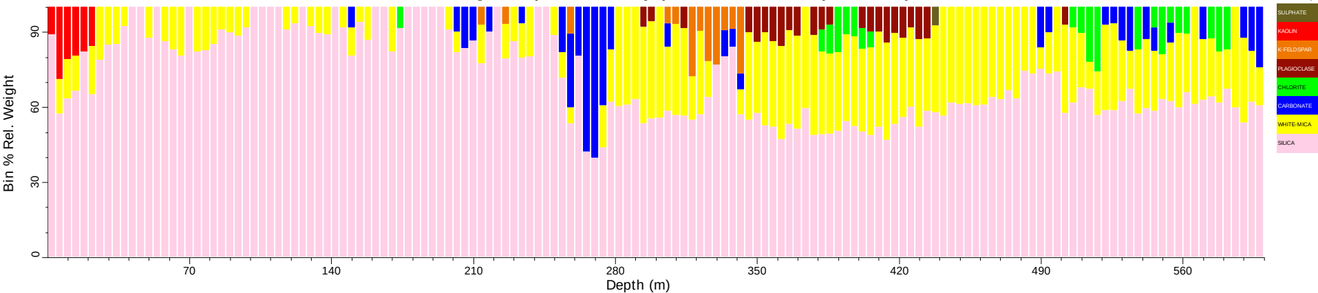
AB62_tsg_tir: Spatial Summary (Bin=4 MinBin=5% ujCLST 7.08)
