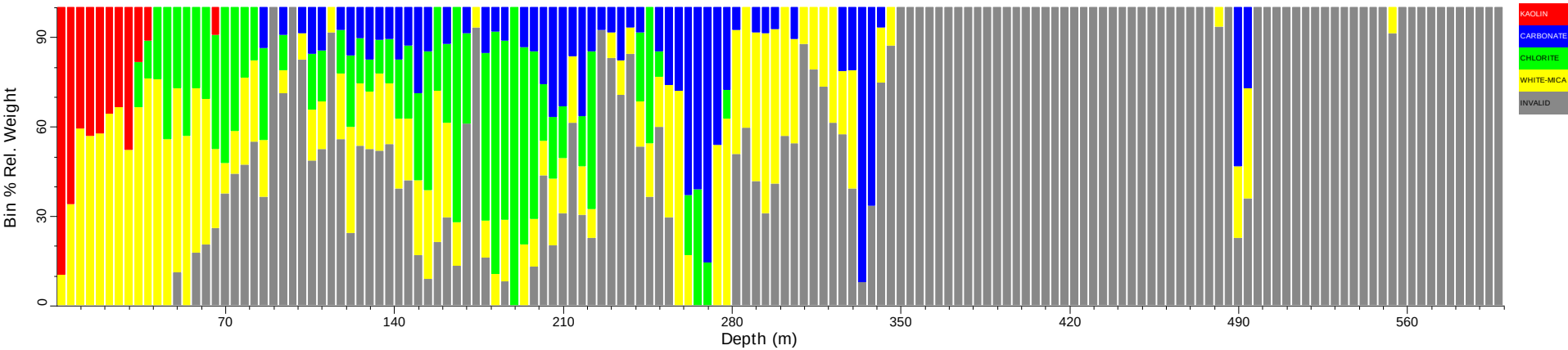
AB62_tsg_tir: Spatial Summary (Bin=4 MinBin=5% ujCLST 7.08)
