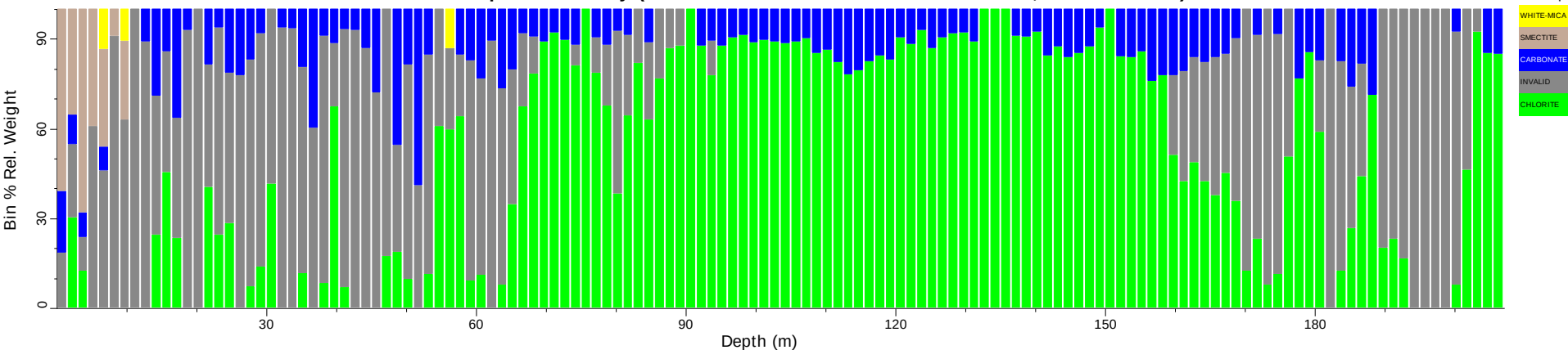
ABDP10_tsg_tir: Spatial Summary (Bin=1.5 MinBin=5% Un-edited sjCLST 7.08, Mineral Subset)
