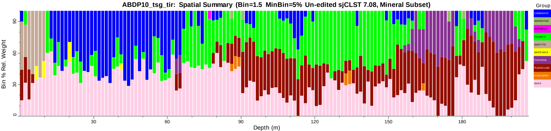
ABDP10_tsg_tir: Spatial Summary (Bin=1.5 MinBin=5% Un-edited sjCLST 7.08, Mineral Subset)
