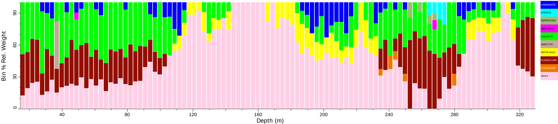
ABDP8_tsg_tir: Spatial Summary (Bin=3 MinBin=5% sjCLST 7.08)
