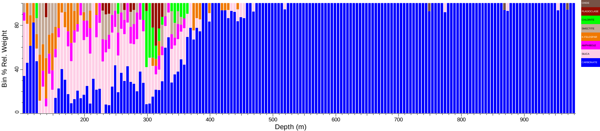
ABDP9_tsg_tir: Spatial Summary (Bin=5 MinBin=5% ujCLST 7.08, Mineral Subset)
