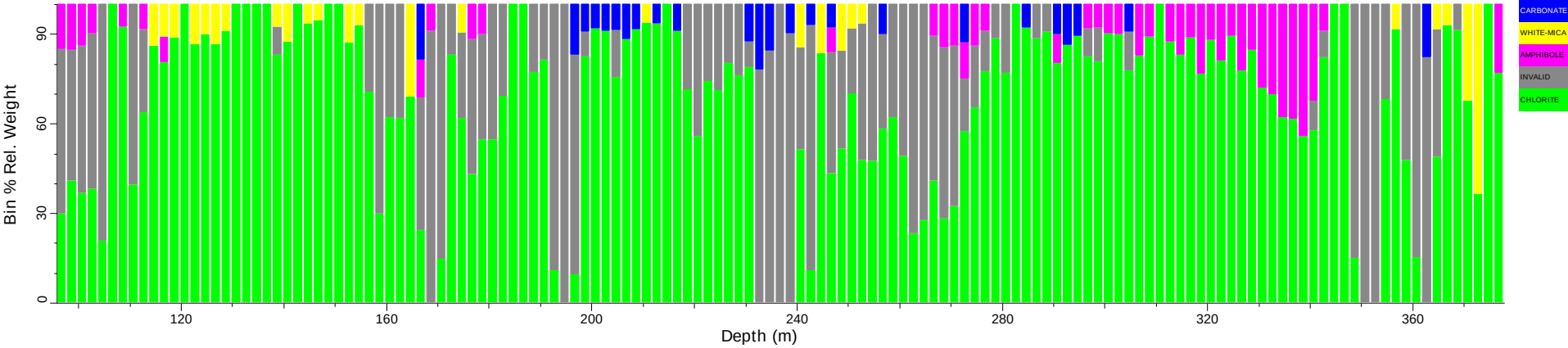
AIDP1_tsg_tir: Spatial Summary (Bin=2 MinBin=5% sjCLST 7.08)
