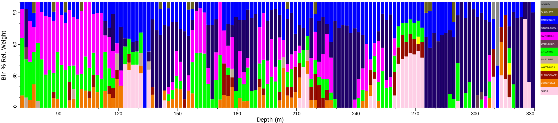
AMDD003_tsg_tir: Spatial Summary (Bin=2 MinBin=5% sjCLST 7.08)
