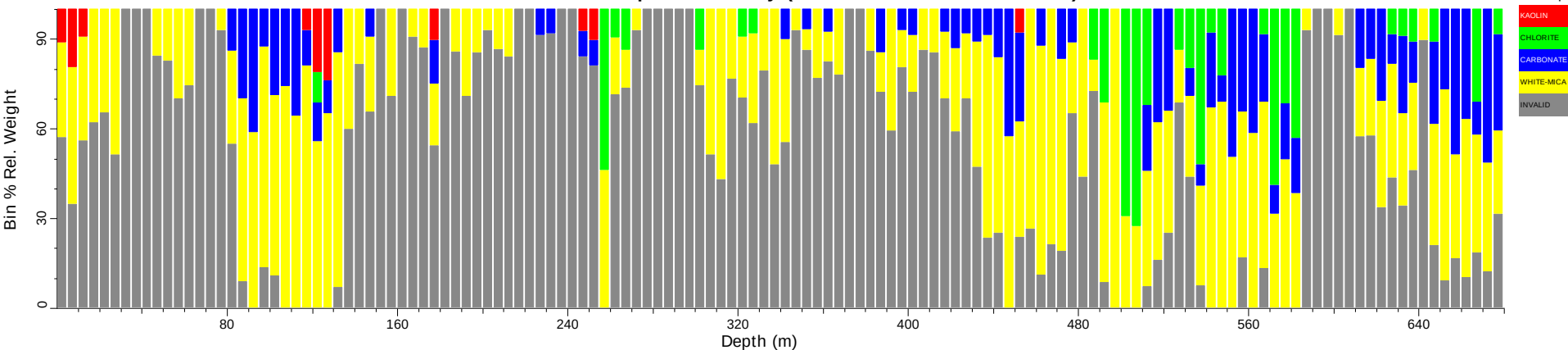
AMODD0028_tsg_tir: Spatial Summary (Bin=5 MinBin=5% ujCLST 7.08)
