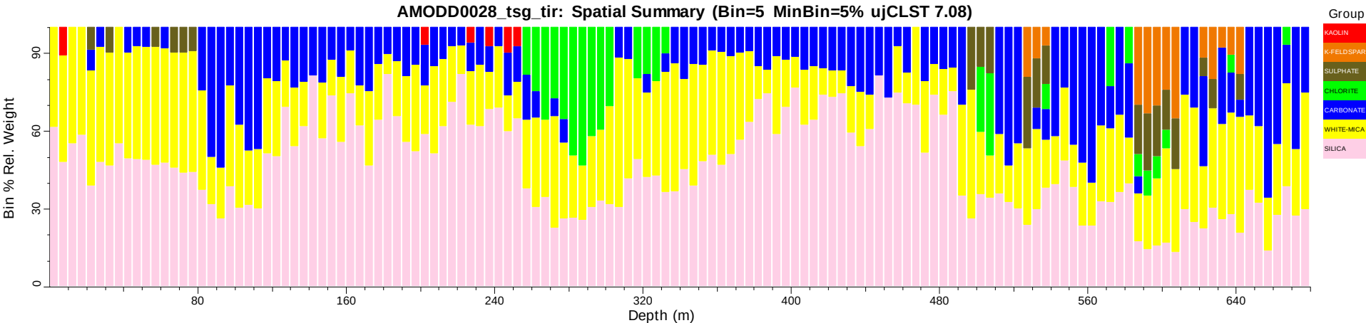
AMODD0028_tsg_tir: Spatial Summary (Bin=5 MinBin=5% ujCLST 7.08)
