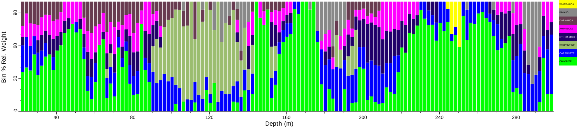
AN15_tsg_tir: Spatial Summary (Bin=2 MinBin=5% ujCLST 7.08, Mineral Subset)
