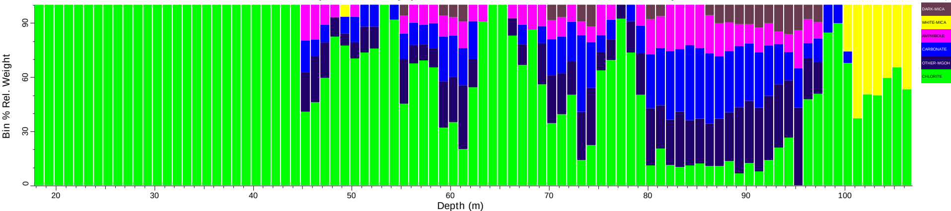
AN7_tsg_tir: Spatial Summary (Bin=1 MinBin=5% ujCLST 7.08, Mineral Subset)
