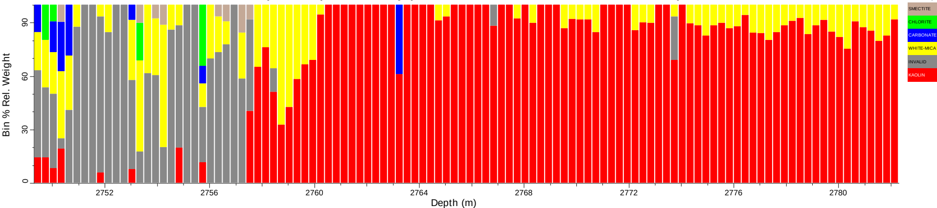
Apium 1_tsg_tir: Spatial Summary (Bin=0.3 MinBin=5% ujCLST 7.08, Mineral Subset)
