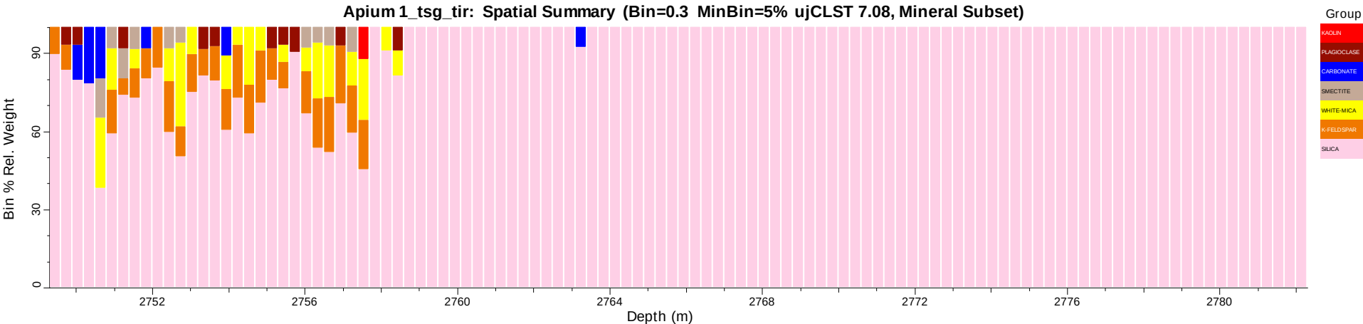
Apium 1_tsg_tir: Spatial Summary (Bin=0.3 MinBin=5% ujCLST 7.08, Mineral Subset)
