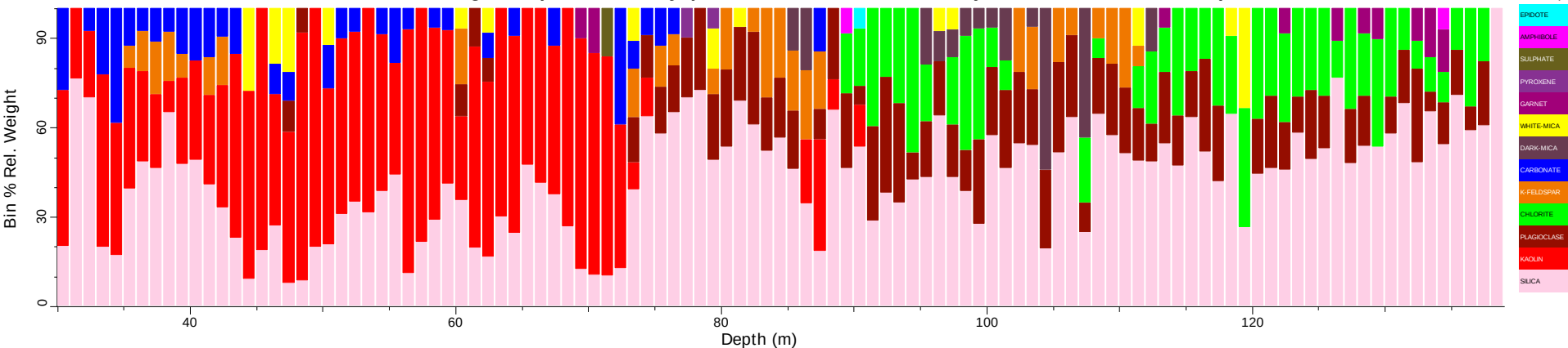
BCDD0002_tsg_tir: Spatial Summary (Bin=1 MinBin=5% Un-edited sjCLST 7.08, Mineral Subset)
