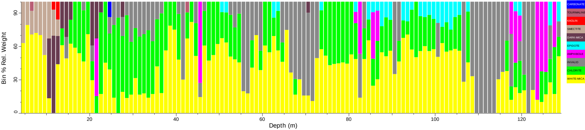
BCDD0004_tsg_tir: Spatial Summary (Bin=1 MinBin=5% Un-edited sjCLST 7.08, Mineral Subset)
