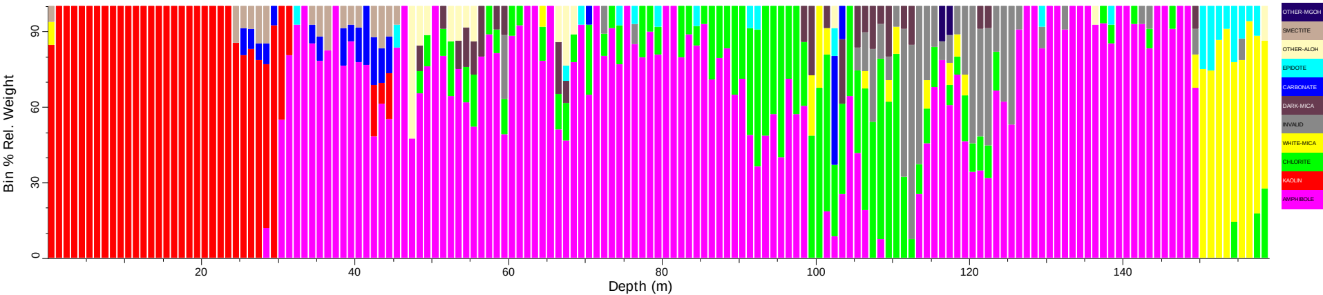
BCM0070_tsg_tir: Spatial Summary (Bin=1 MinBin=5% ujCLST 7.08, Mineral Subset)
