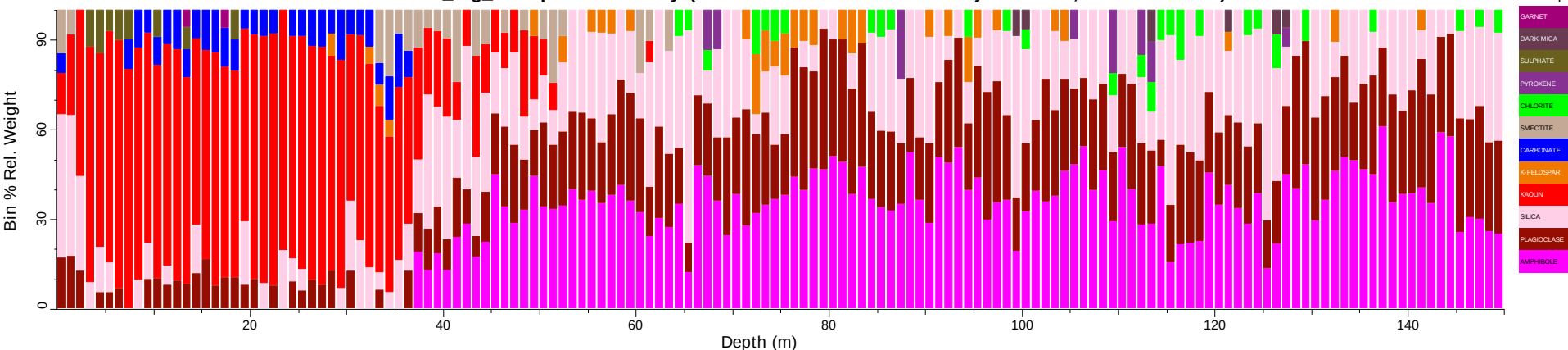
BCM0071_tsg_tir: Spatial Summary (Bin=1 MinBin=5% Un-edited sjCLST 7.08, Mineral Subset)
