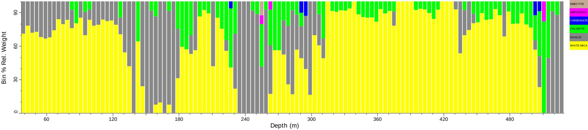
BDD003_tir: Spatial Summary (Bin=4 MinBin=5% sjCLST 7.08)
