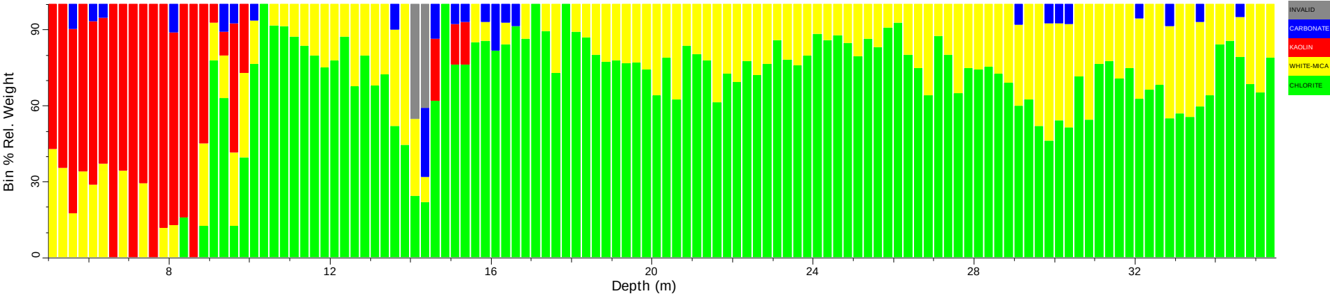
BDD2_tsg_tir: Spatial Summary (Bin=0.25 MinBin=5% sjCLST 7.08)
