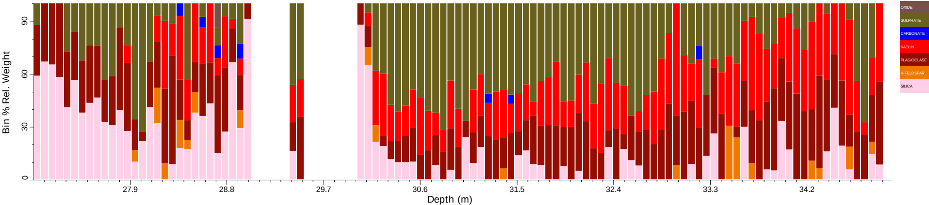
BH15_tsg_tir: Spatial Summary (Bin=0.07 MinBin=5% sjCLST 7.08)
