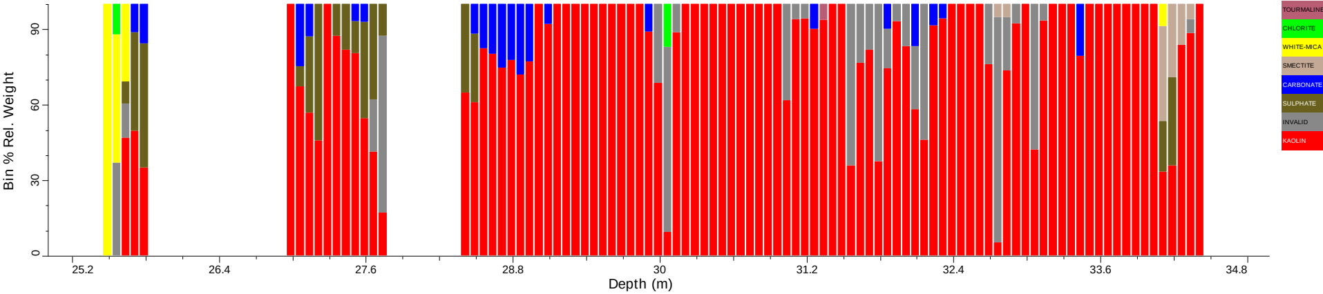
BH16_tsg_tir: Spatial Summary (Bin=0.075 MinBin=5% sjCLST 7.08)
