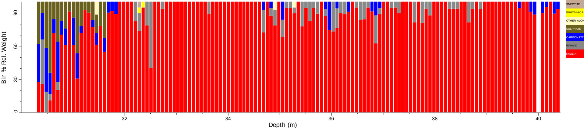
BH18_tsg_tir: Spatial Summary (Bin=0.075 MinBin=5% sjCLST 7.08)
