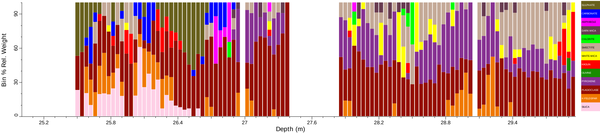
BH23_tsg_tir: Spatial Summary (Bin=0.04 MinBin=5% sjCLST 7.08)
