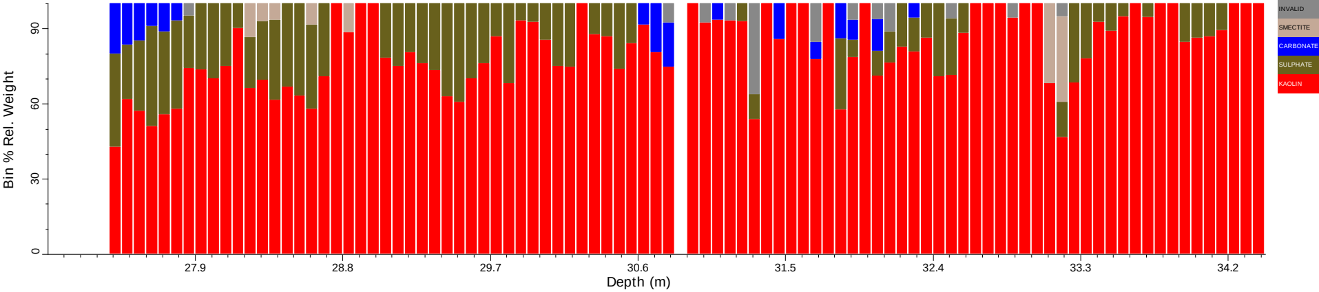
BH26_tsg_tir: Spatial Summary (Bin=0.075 MinBin=5% sjCLST 7.08)
