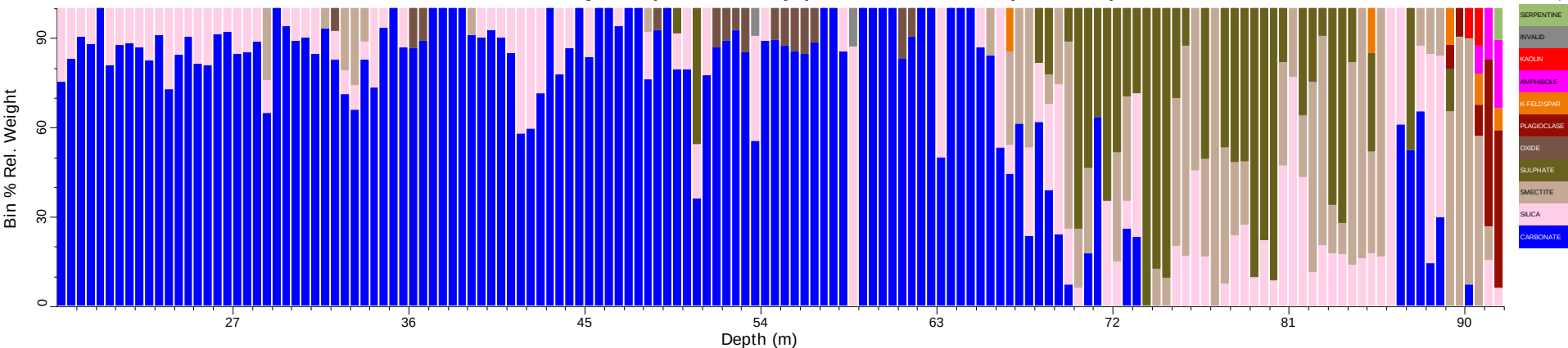
BLRCD006_tsg_tir: Spatial Summary (Bin=0.5 MinBin=5% ujCLST 7.08)
