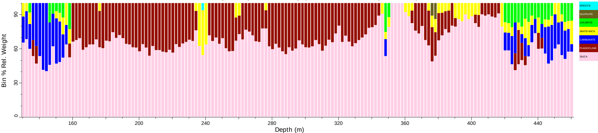
BOD202_tsg_tir: Spatial Summary (Bin=2 MinBin=5% ujCLST 7.08)
