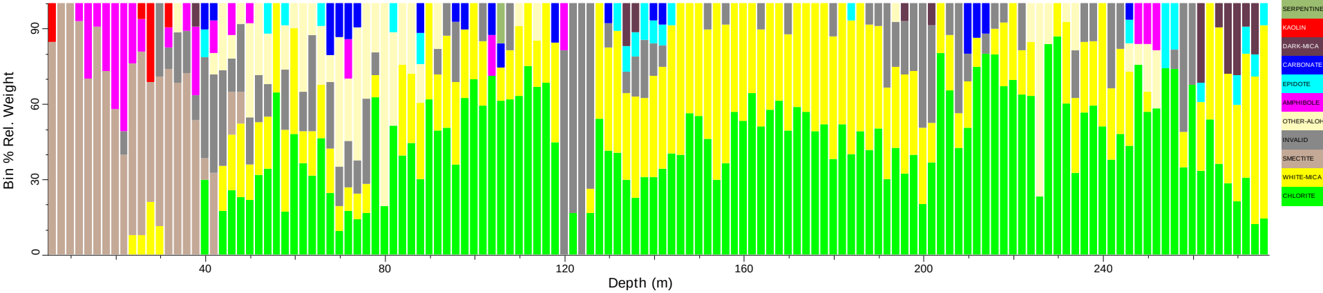
BSDD030_tsg_tir: Spatial Summary (Bin=2 MinBin=5% Un-edited sjCLST 7.08, Mineral Subset)
