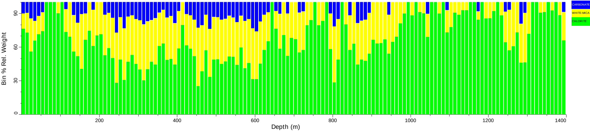
CCUD001_tsg_tir: Spatial Summary (Bin=10 MinBin=5% sjCLST 7.08)
