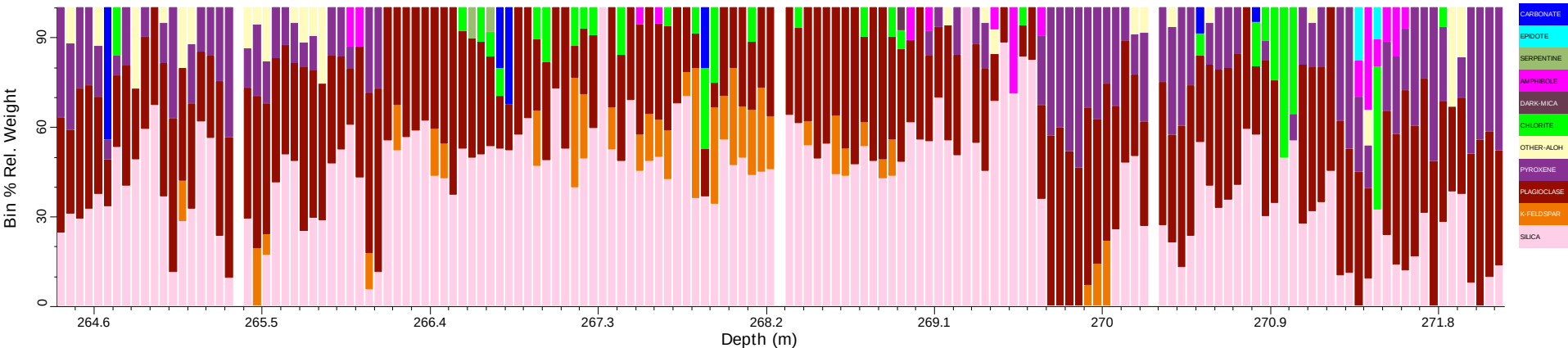
CD1_tsg_tir: Spatial Summary (Bin=0.05 MinBin=5% sjCLST 7.08)
