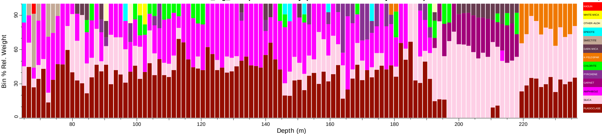
CFDD001_tsg_tir: Spatial Summary (Bin=1.5 MinBin=5% sjCLST 7.08)
