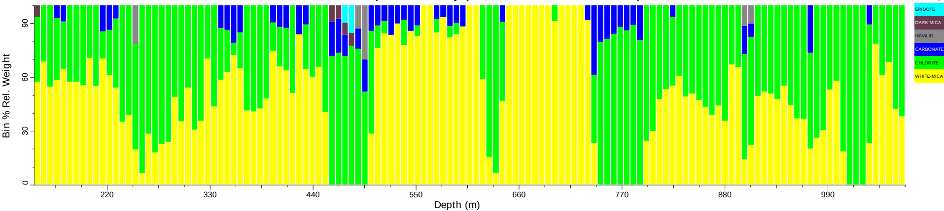
CUDD001_tsg_tir: Spatial Summary (Bin=7 MinBin=5% ujCLST 7.08)
