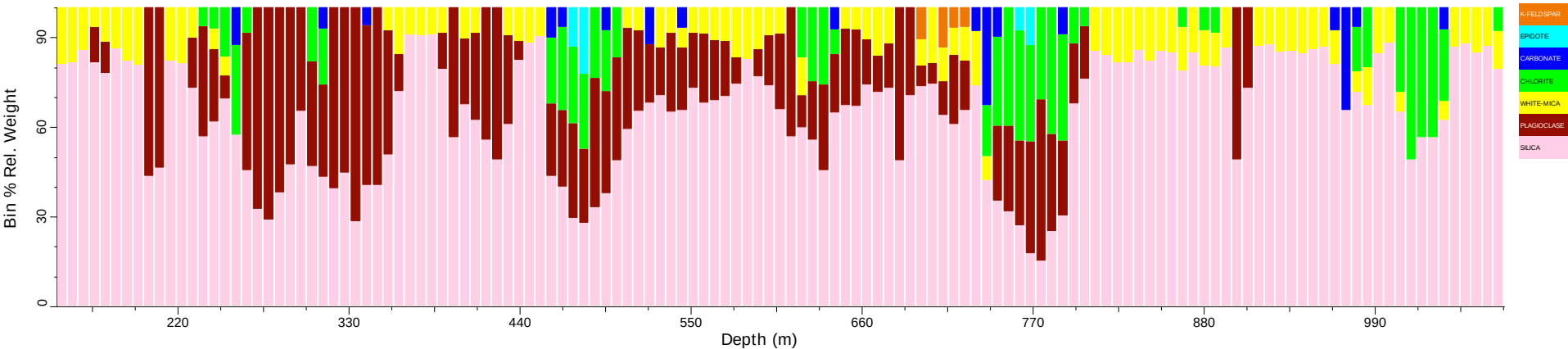
CUDD001_tsg_tir: Spatial Summary (Bin=7 MinBin=5% ujCLST 7.08)
