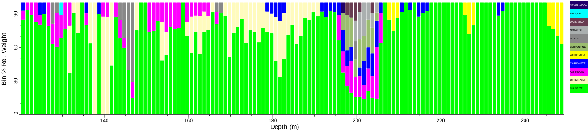
CXDD003_tsg_tir: Spatial Summary (Bin=1 MinBin=5% ujCLST 7.08)
