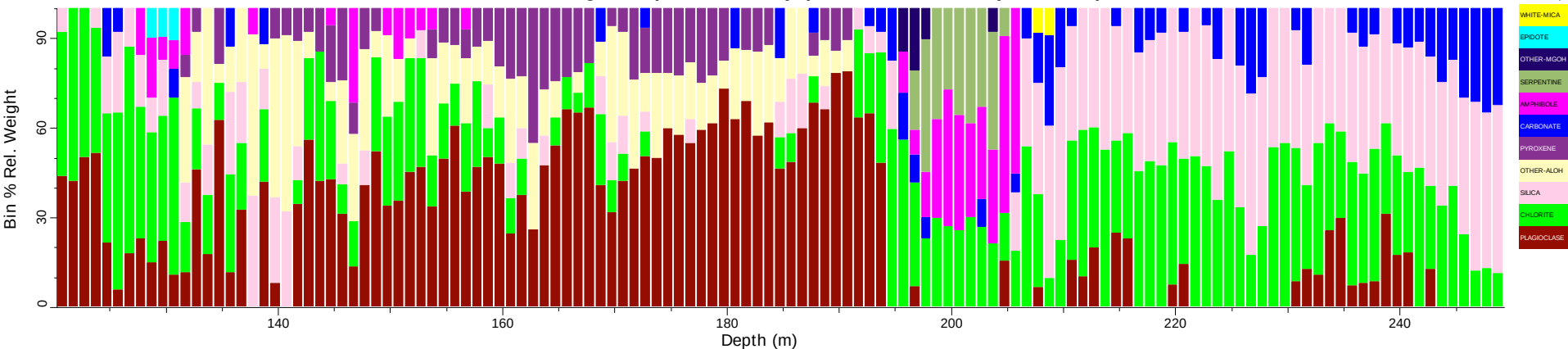
CXDD003_tsg_tir: Spatial Summary (Bin=1 MinBin=5% ujCLST 7.08)
