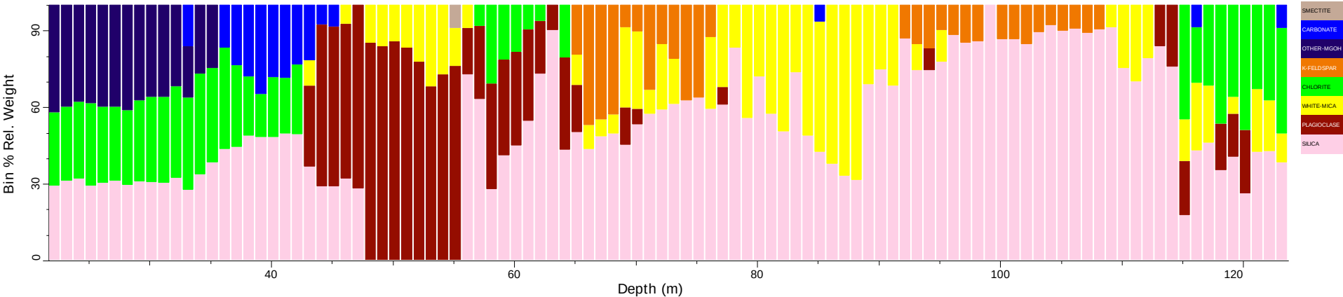
93HSDDH2_tsg_tir: Spatial Summary (Bin=1 MinBin=5% ujCLST 7.08)
