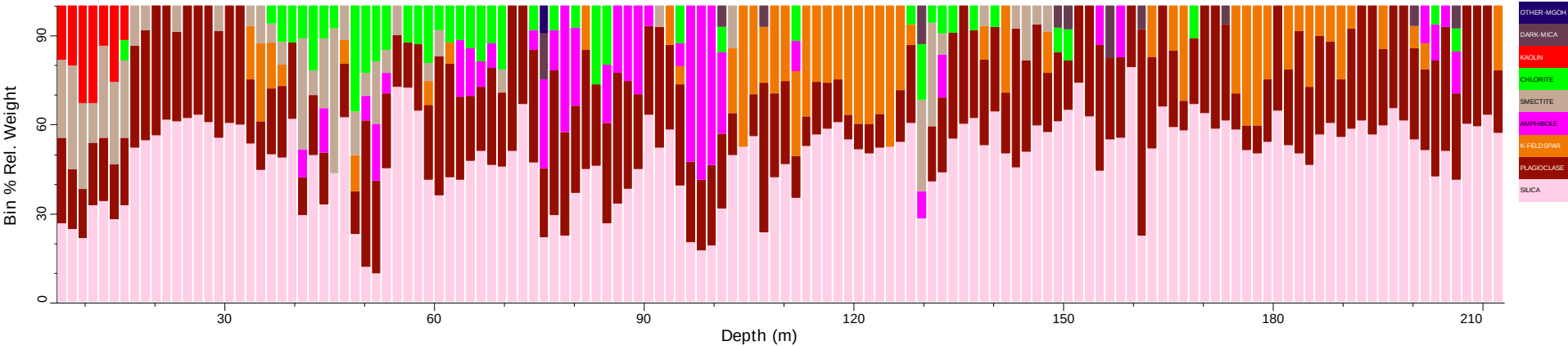
DDB17_tsg_tir: Spatial Summary (Bin=1.5 MinBin=5% sjCLST 7.08)
