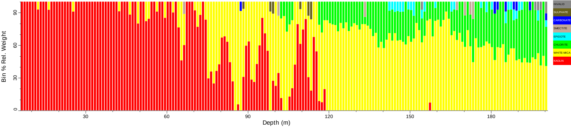
DDB9_tsg_tir: Spatial Summary (Bin=1 MinBin=5% sjCLST 7.08)
