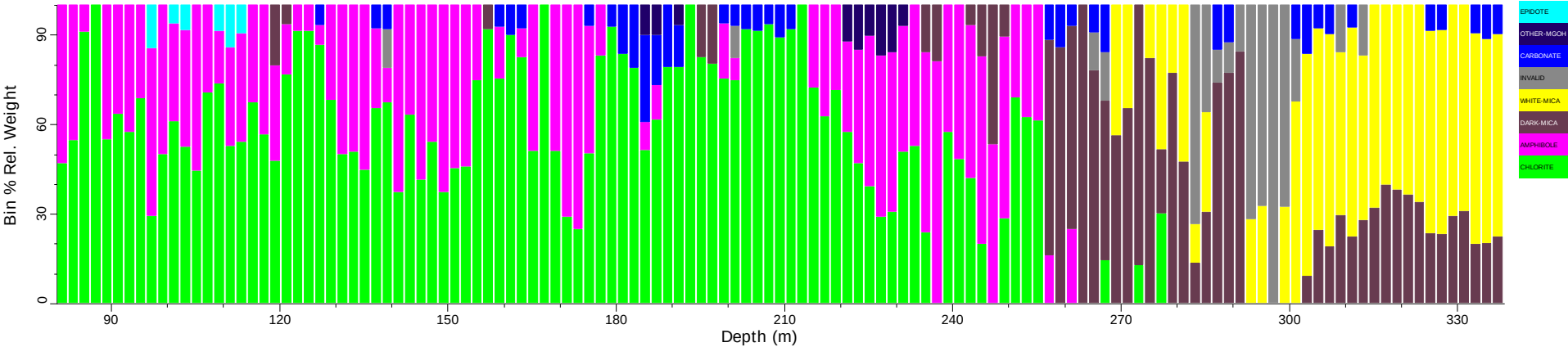
DGDH009_tsg_tir: Spatial Summary (Bin=2 MinBin=5% sjCLST 7.08)
