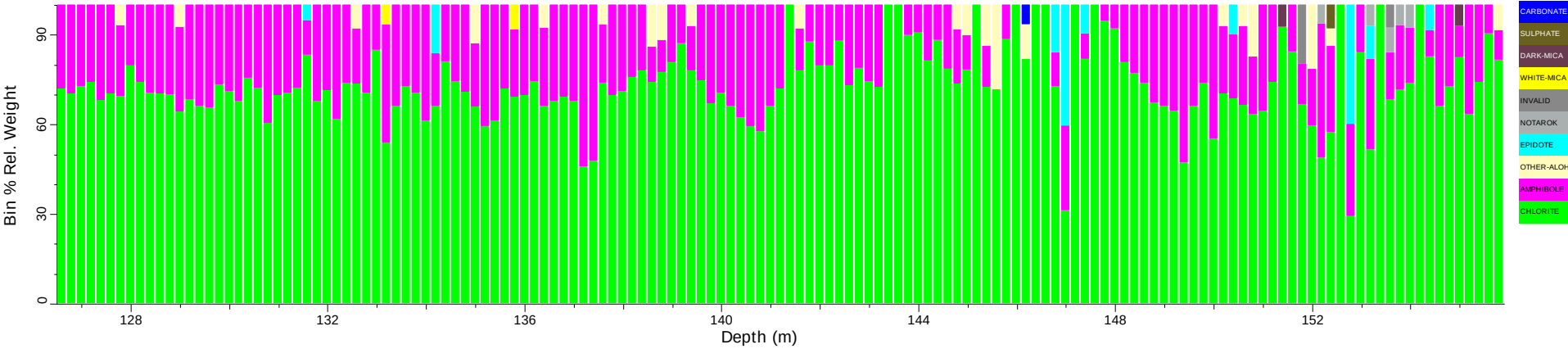
EC173D_tsg_tir: Spatial Summary (Bin=0.2 MinBin=5% sjCLST 7.08)
