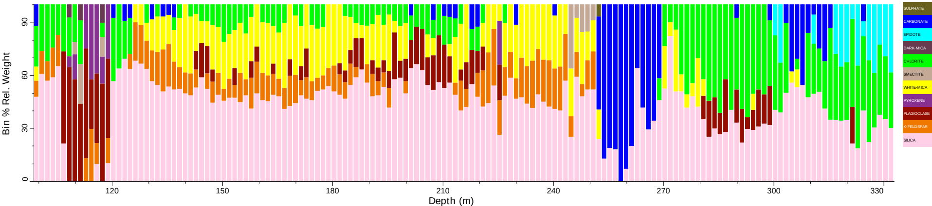
EGD002_tsg_tir: Spatial Summary (Bin=1.5 MinBin=5% sjCLST 7.08)
