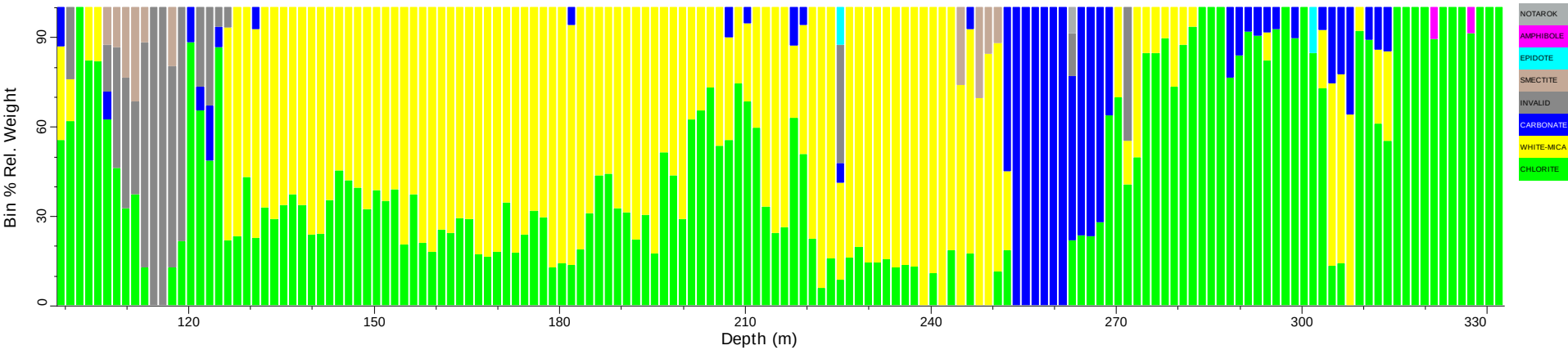
EGD002_tsg_tir: Spatial Summary (Bin=1.5 MinBin=5% sjCLST 7.08)
