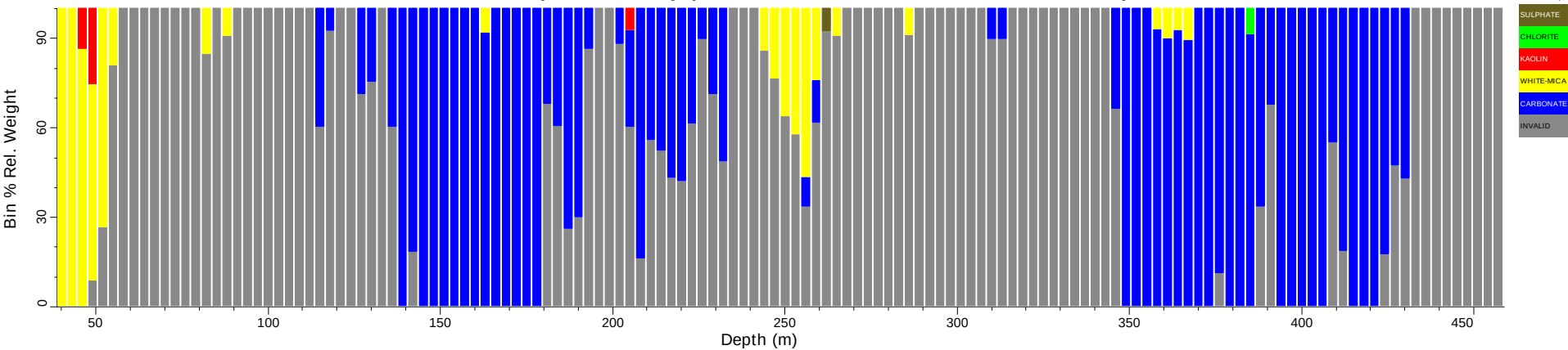
EPT057_tsg_tir: Spatial Summary (Bin=3 MinBin=5% ujCLST 7.08, Mineral Subset)
