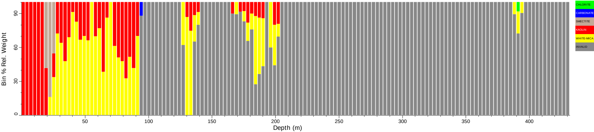
EPT1174_tsg_tir: Spatial Summary (Bin=3 MinBin=5% ujCLST 7.08)
