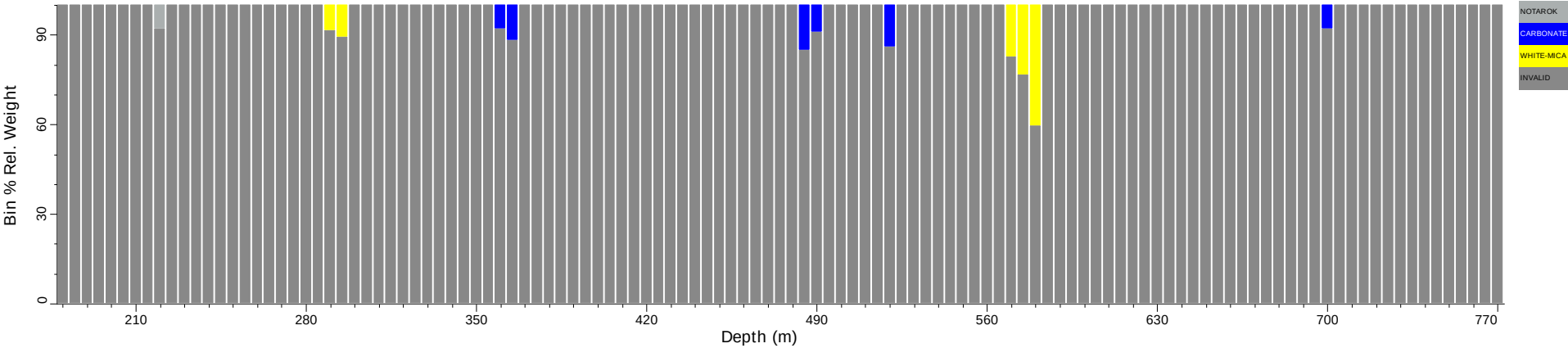
EPT1702_tsg_tir: Spatial Summary (Bin=5 MinBin=5% sjCLST 7.08)
