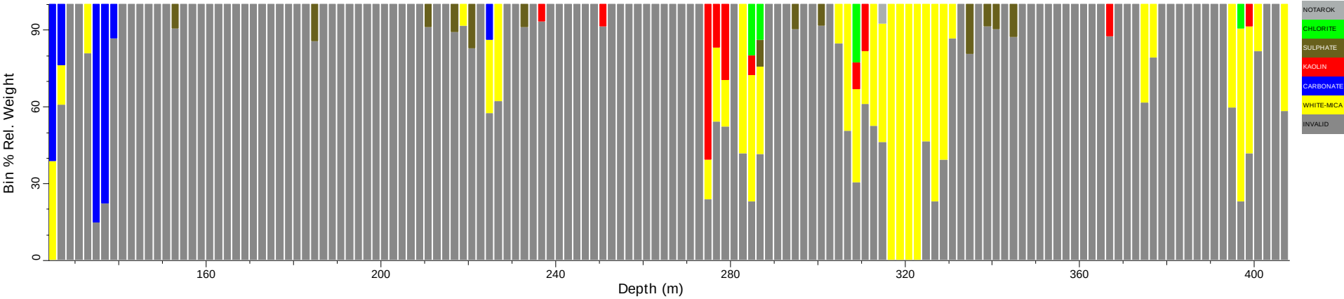
EPT2279_tir: Spatial Summary (Bin=2 MinBin=5% sjCLST 7.08)
