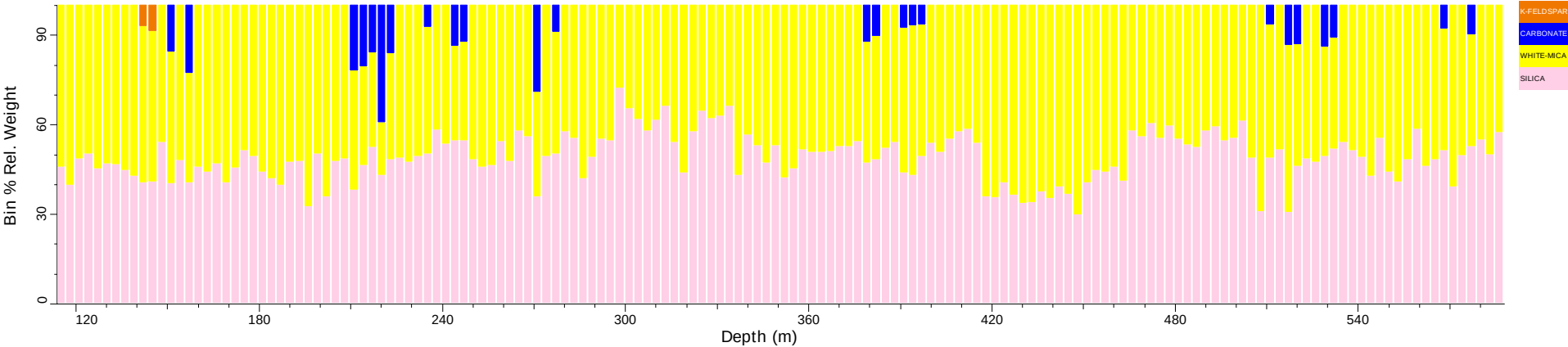
EPT2299_tsg_tir: Spatial Summary (Bin=3 MinBin=5% sjCLST 7.08)
