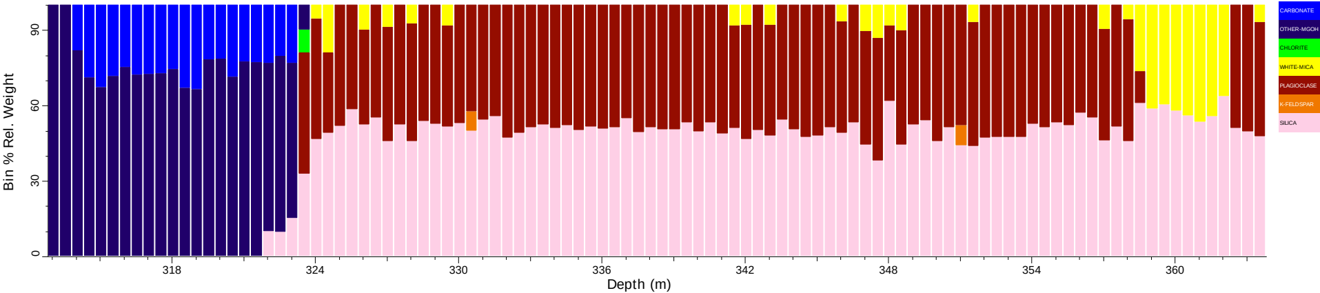
ERCD145_tsg_tir: Spatial Summary (Bin=0.5 MinBin=5% sjCLST 7.08)
