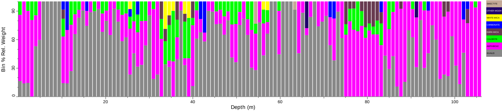
FMM397_tsg_tir: Spatial Summary (Bin=0.9 MinBin=5% ujCLST 7.08)
