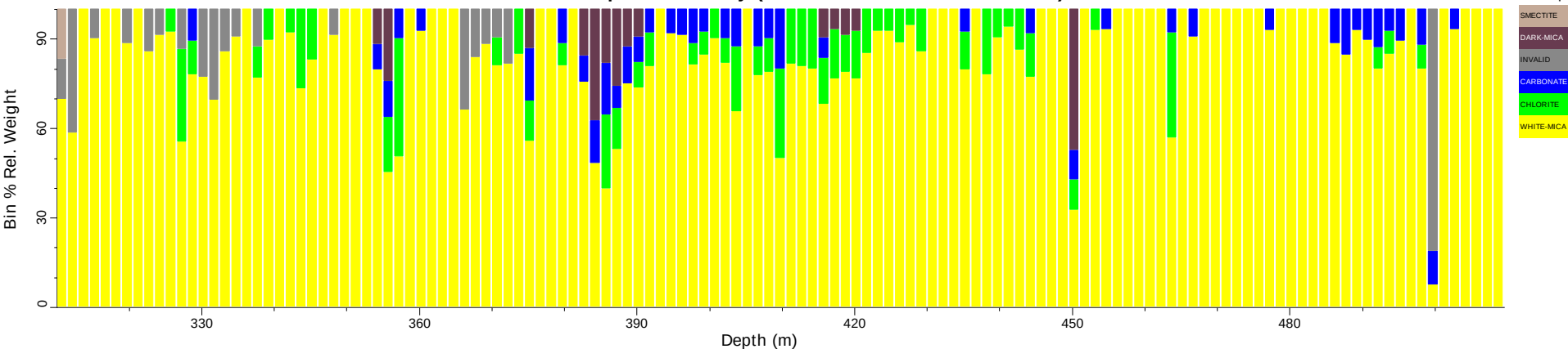
FOR012_tsg_tir: Spatial Summary (Bin=1.5 MinBin=5% ujCLST 7.08)
